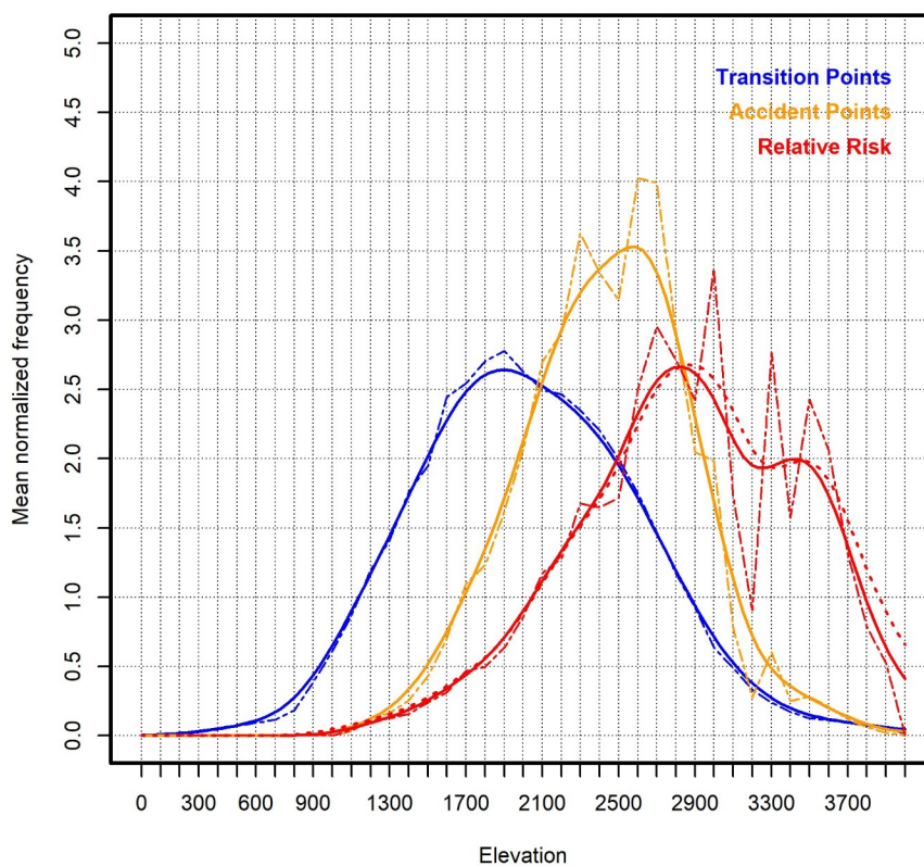
DISTRIBUTION: Elevation
