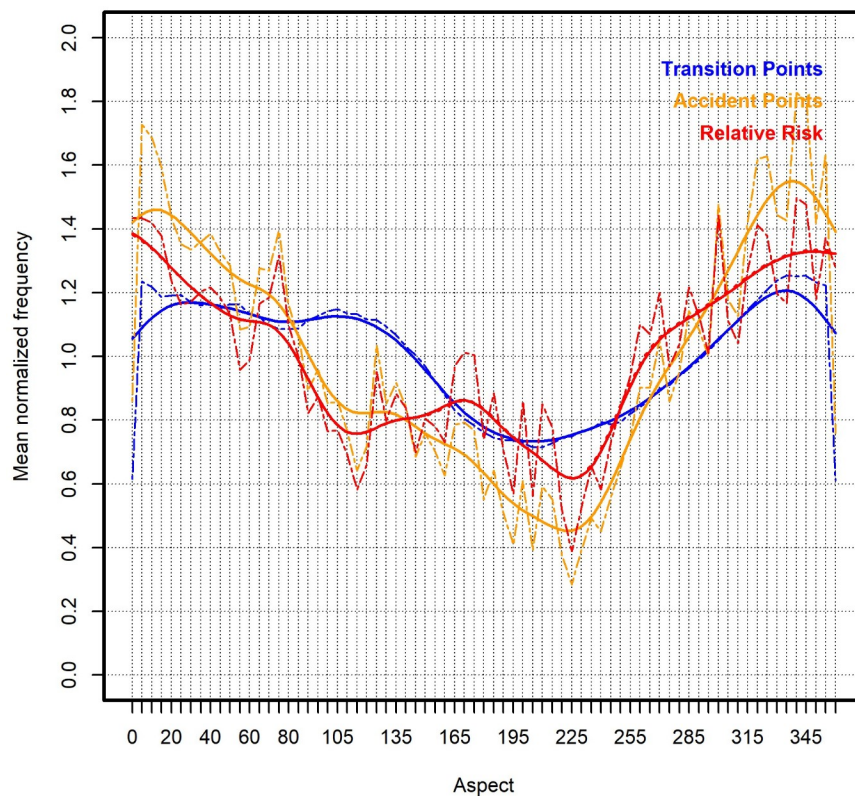
DISTRIBUTION: Aspect
