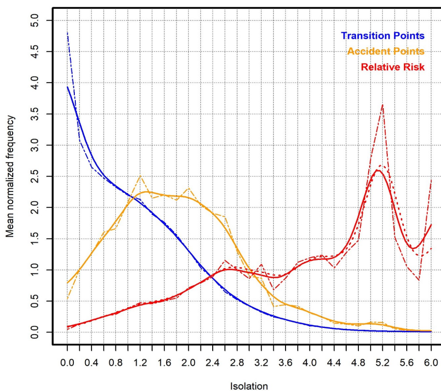
DISTRIBUTION: Isolation
